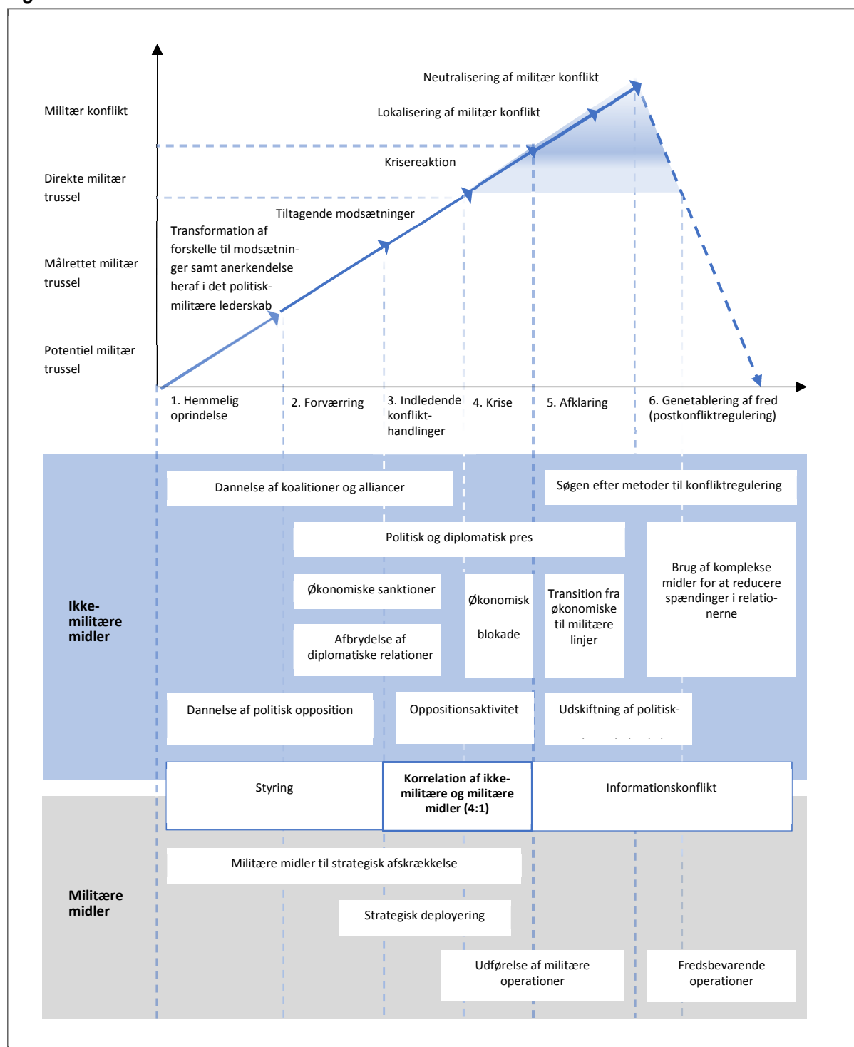
Figur 4: Gerasimov-modellen
